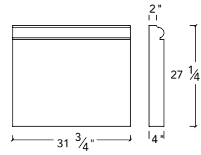
W-27-32 Wainscot
