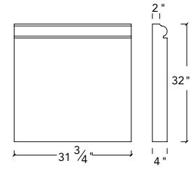
W-32-32 Wainscot
