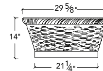
P-BW Basket Weave
