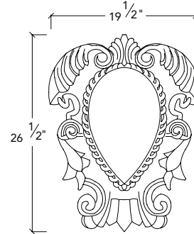
DP-1 Depth 4"
