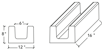
SC-3 Scupper
