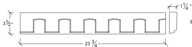
#4 Dentil Frieze
