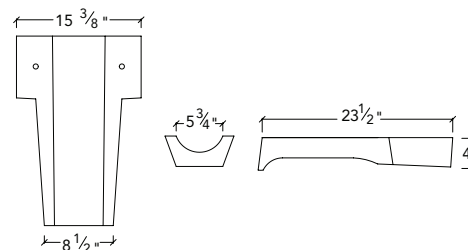
SC-6 Scupper
