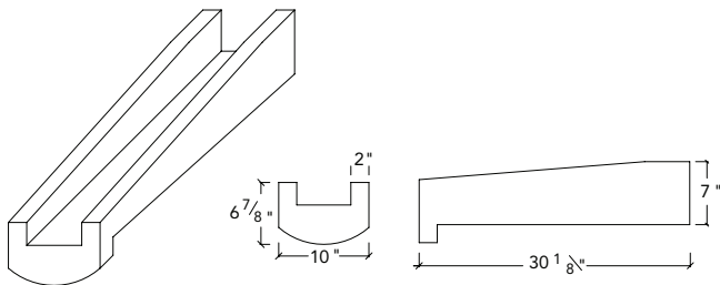
SC-5 Scupper
