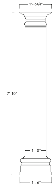
Split GFRC Column
