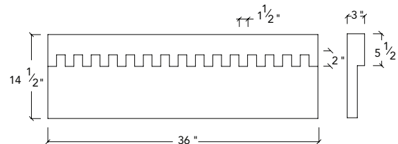
#2 Dentil Frieze
