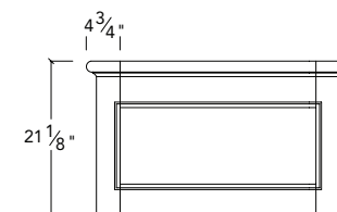
P-RC Rectangular Planter Available in various lengths
