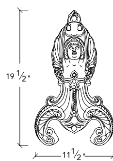
Angel Depth 2 3/4"
